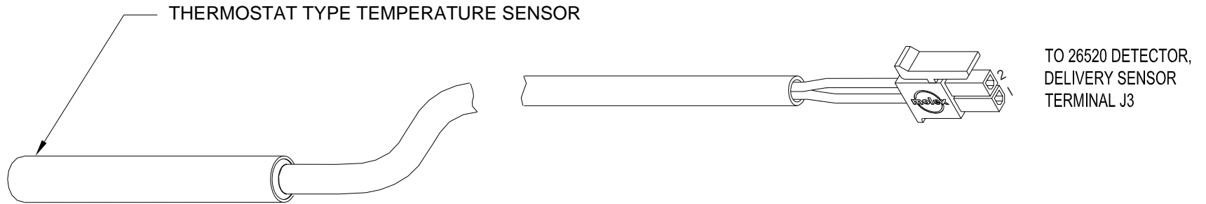
21468 TEMPERATURE SENSOR
