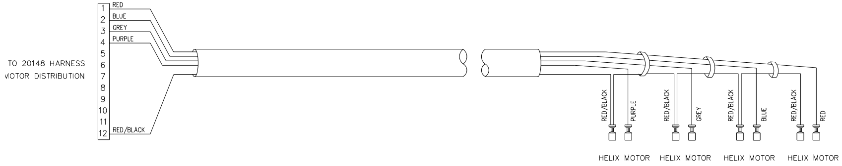
21584, HARNESS, 1.5" HELIX TRAY (OPTIONAL)
