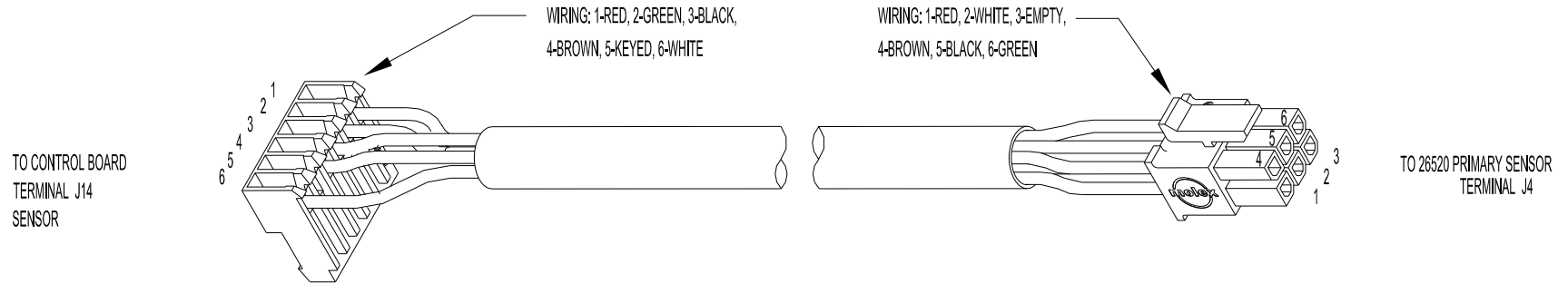
21425 HARNESS, DELIVERY SENSOR DETECTOR/CONTROL
