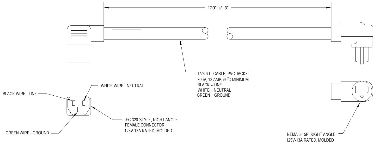
20142, POWER CORD ASSEMBLY, 115V DOMESTIC
