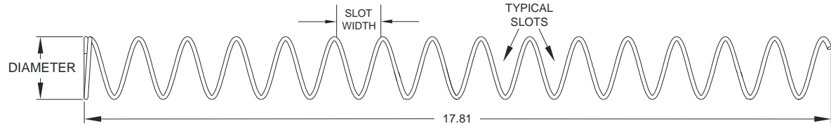
TYPICAL 1.5 HELIX TRAY SMALL HELIX
