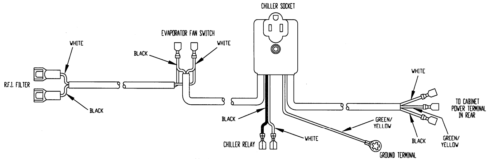
21484, HARNESS, POWER DISTRIBUTION, INTEGRAL SOCKET, ON/OFF SWITCH
