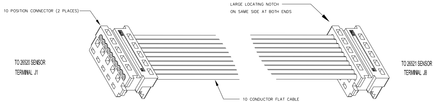
21426 HARNESS, DELIVERY SENSOR DETECTOR/EMITTER
