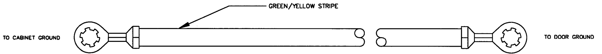
20156-01, HARNESS, GROUND
