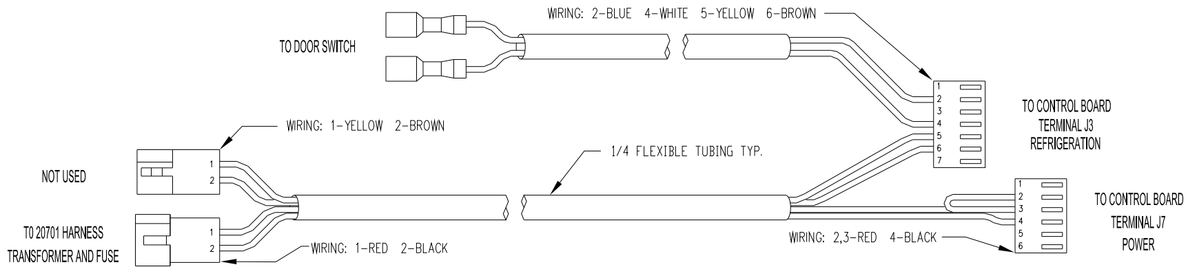
21591, HARNESS, CONTROL POWER AND DOOR SWITCH
