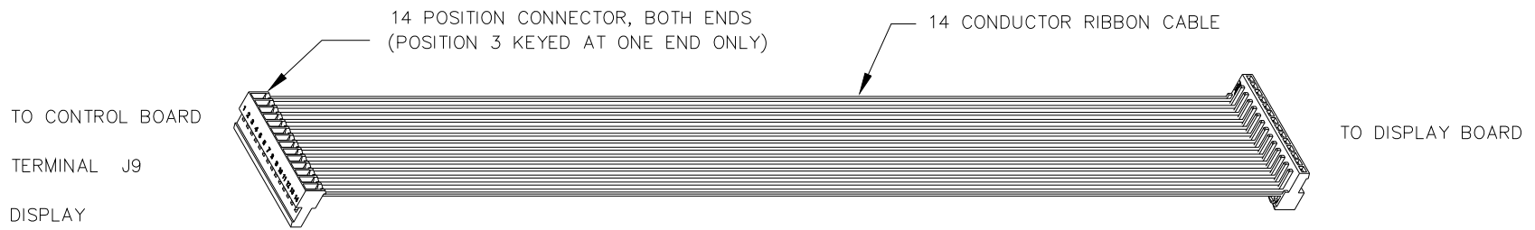
24015 HARNESS, DISPLAY
