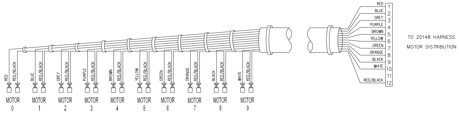
20147, HARNESS, TRAY, 10 COLUMN
