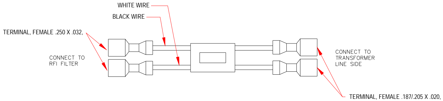
23624, HARNESS, TRANSFORMER, NO BALLAST
